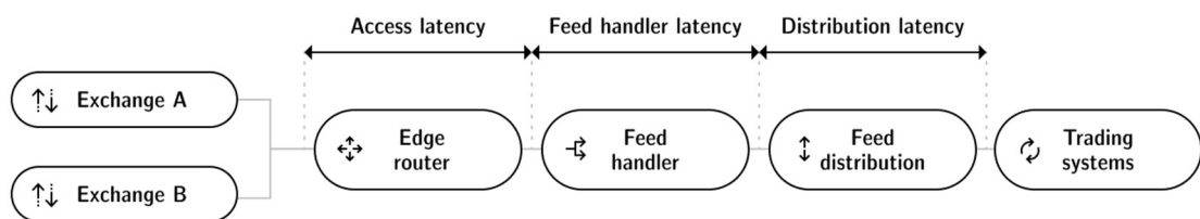
The use of a unified protocol for receiving market data from different sources
